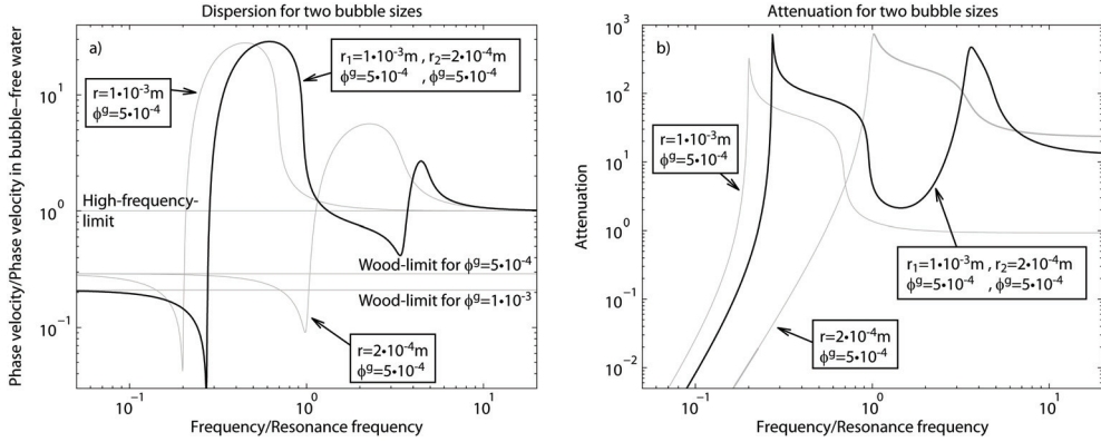
Fig. 5. Dispersion (a) and frequency-dependent attenuation (b) for water containing gas bubbles with two different radii r_1=1\cdot 10^{-3}\text{m} and r_2=2\cdot 10^{-4}\text{m} . Material parameters are given in Table 1 and Table 2. Plotted in light gray for comparison are the dispersion and the frequency-dependent attenuation of two models containing only either of the two bubble sizes with their respective volume fraction. The frequency is normalized with the resonance frequency of the larger bubble and the phase velocity is normalized with the phase velocity in bubble-free water, i.e. with the high-frequency-limit.
