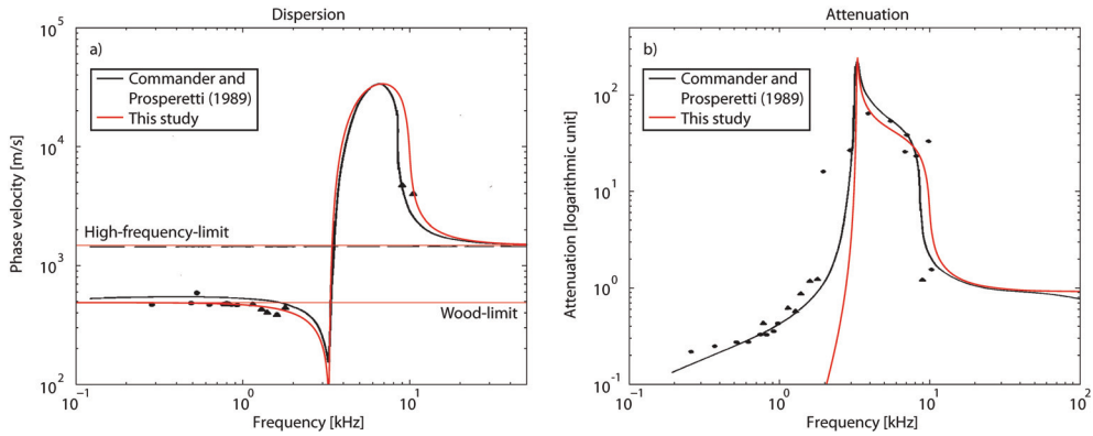
Fig. 7. Phase velocity dispersion (a) and frequency-dependent attenuation (b) for a model with one gas bubble size r=9.94 \times 10^{-4} \text{m} and a gas volume fraction \phi=3.77 \times 10^{-4} . Plotted in black are Figures 8 and 1 of Commander and Prosperetti (1989). Data points are also taken from Commander and Prosperetti (1989), who took the data from Silberman (1957). All values are plotted as absolute values. In b), attenuation is plotted as a logarithmic unit, because in Commander and Prosperetti (1989) the attenuation is given in dB/cm.
