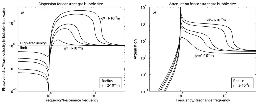
Fig. 4. Dispersion (a) and frequency-dependent attenuation (b) for water containing gas bubbles with a fixed radius r = 2 \cdot 10^{-4} \text{ m} . Material parameters are given in Table 1. While the gas bubble size is kept constant, the gas volume fraction is different for the different lines ( \phi^g = \{1 \cdot 10^{-4}, 5 \cdot 10^{-4}, 1 \cdot 10^{-3}, 5 \cdot 10^{-3}, 1 \cdot 10^{-2}\} ). The frequency is normalized with the resonance frequency and the phase velocity is normalized with the phase velocity in bubble-free water, i.e. with the high-frequency-limit.
