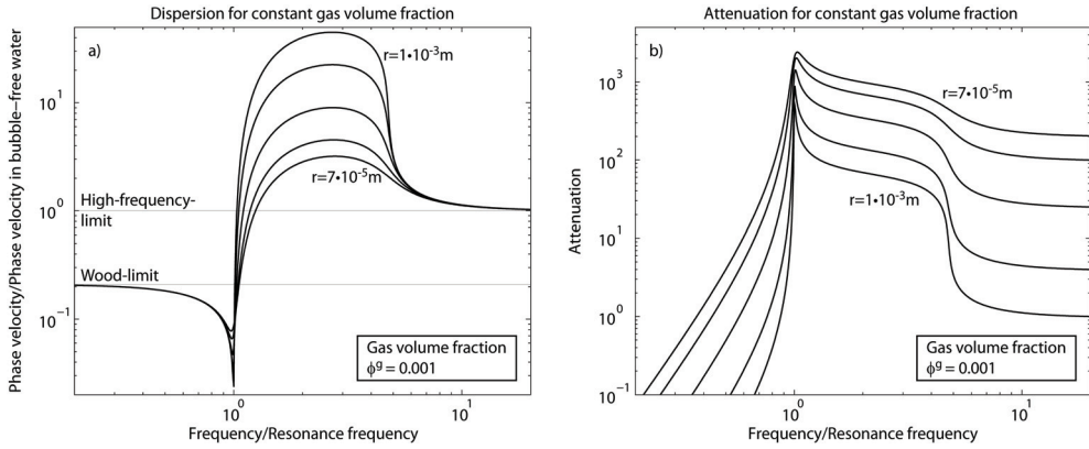
Fig. 3. Dispersion (a) and frequency-dependent attenuation (b) for water containing gas with a fixed volume fraction \phi^g = 0.001 . Material parameters are given in Table 1. While the gas volume fraction is kept constant, for each curve the gas volume is contained in bubbles with equal radius (in meter) r = \{7 \cdot 10^{-5}, 1 \cdot 10^{-4}, 2 \cdot 10^{-4}, 5 \cdot 10^{-4}, 1 \cdot 10^{-3}\} . The frequency is normalized with the resonance frequency and the phase velocity is normalized with the phase velocity in bubble-free water, i.e. with the high-frequency-limit.
