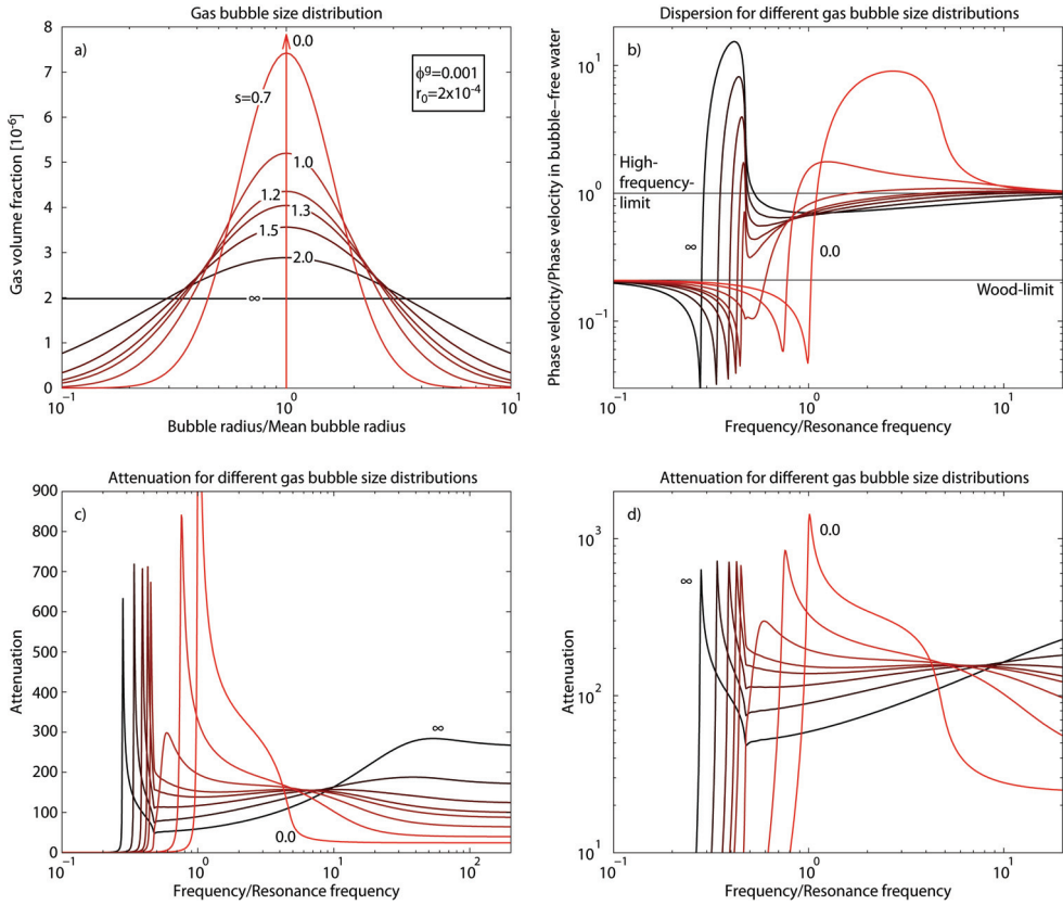
Fig. 6. a) Gas volume fraction versus bubble radius. The bubble radius is normalized with r_0 = 2 \times 10^{-4} \text{ m} . Along these curves, 501 discrete values are picked at equally spaced values for the logarithm of the bubble radius, i.e. the curves are discrete probability functions, rather than continuous ones. The sum of all 501 values is equal to \phi^g = 0.001 . Labels correspond to the values of parameter s in Equation (27). The curve with label "0.0" corresponds to a model with only one bubble size. b), c) and d) Dispersion and two different representations of the frequency-dependent attenuation for water containing gas with a fixed volume fraction \phi^g = 0.001 and with bubble size distributions shown in a). Labels are only given for the end member curves. All other curves correspond to the curves labeled in a). Material parameters are given in Table 1. The frequency is normalized with the resonance frequency and the phase velocity is normalized with the phase velocity in bubble-free water, i.e. with the high-frequency-limit.
