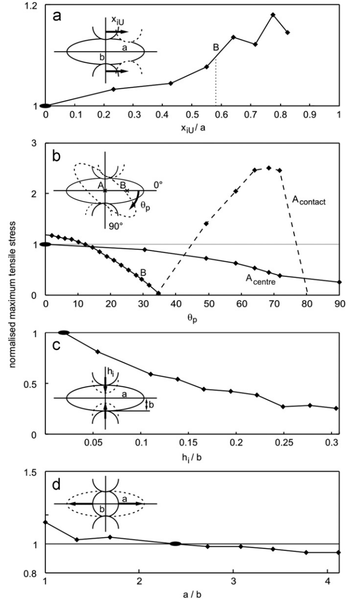
Fig. 9. Maximum tensile stress inside the numerical domain for different loading configurations and for constant displacement u(x_i, y_i) . All results are normalised to the standard loading configuration, which is indicated by a black ellipse.
