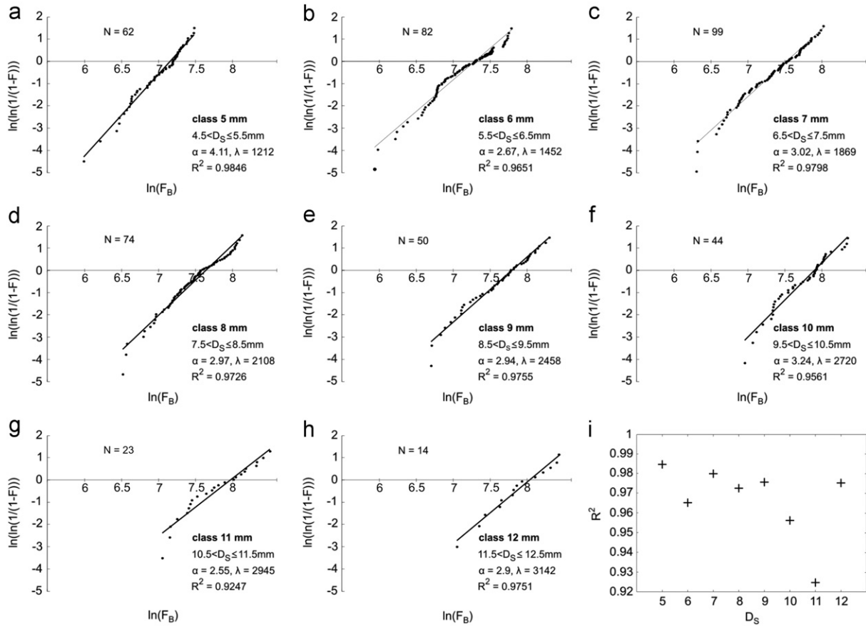
Fig. 6. Cumulative probability for eight grain size classes (a)–(h), calculated from median ranking for breakage load using the linearised two-parameter Weibull distribution [\ln(\ln(1/(1-F)))] . The solid lines represent the best linear fit for the data of each class. (i) Summary of the coefficients of determination of all classes.
