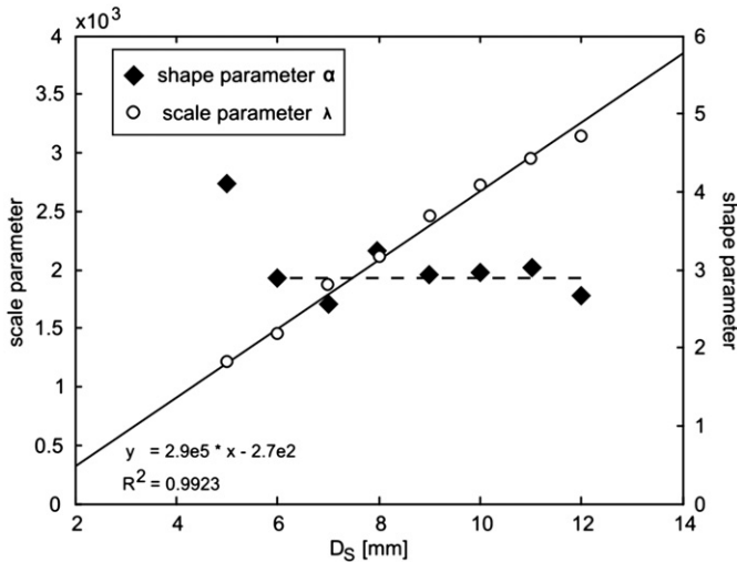
Fig. 7. Scale and shape parameters of the Weibull distribution vs. size class. The solid line is a linear regression to the class mean values of the scale parameter. The fitted dashed line indicates a fairly constant shape parameter for the classes above 5 mm.
